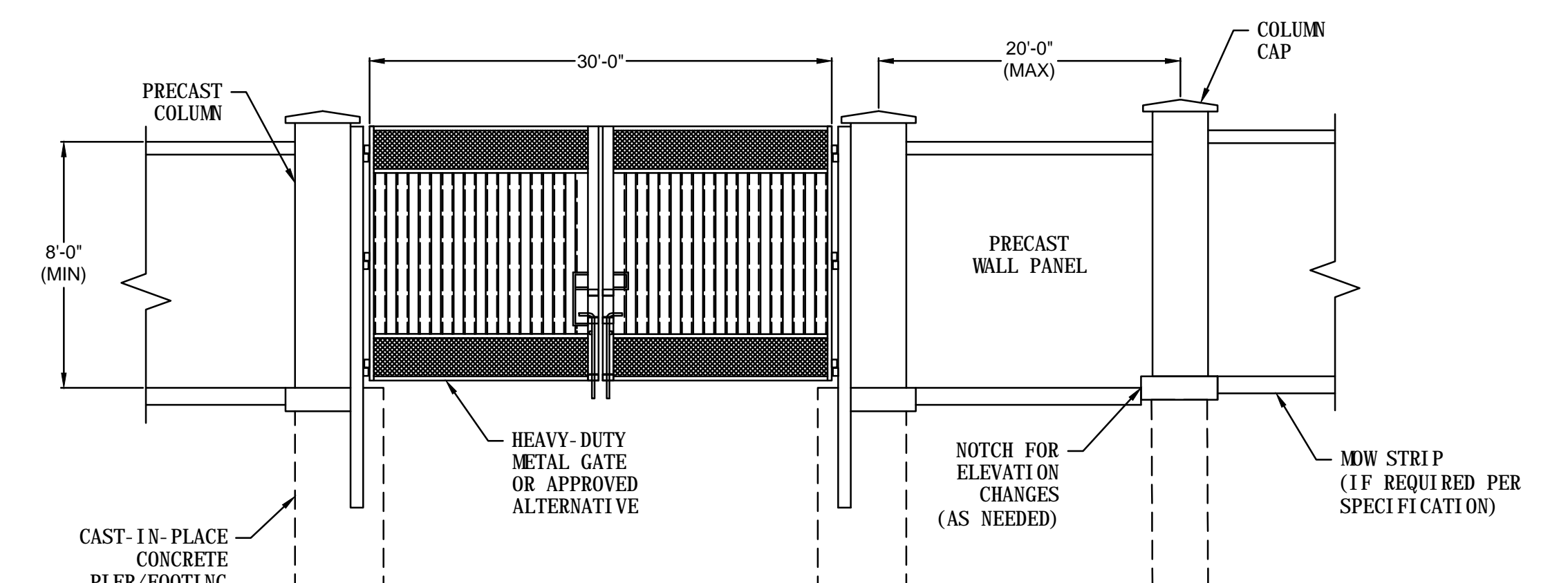
ELEVATION (PRECAST CONCRETE)
